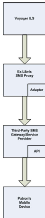
Figure 13-1. Components/Path for Voyager SMS Notices Sent
