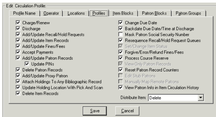
Figure 7-1. Discharge on the Profiles Tab
