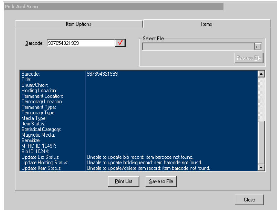
Figure 12-5. Processing Report when the Item Barcode Is Not Found
