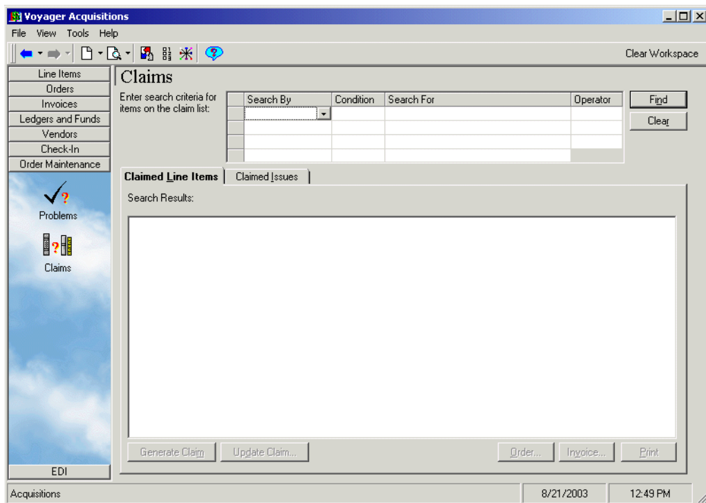
Figure 11-11. Claims workspace
