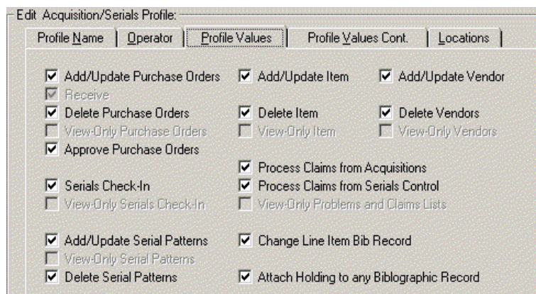
Figure 6-73. Profile Values tab
