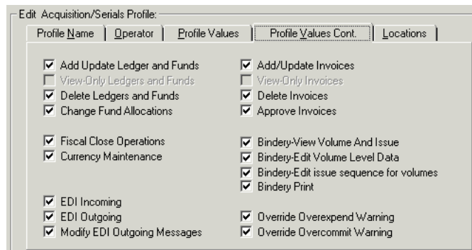
Figure 8-44. Profile Values Cont. tab
