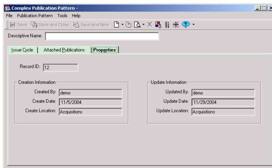
Figure 8-55. Properties tab
