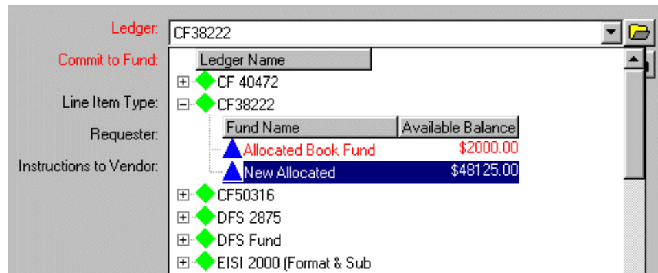
Figure 6-68. Ledger/Fund hierarchy displayed in the Ledger field
