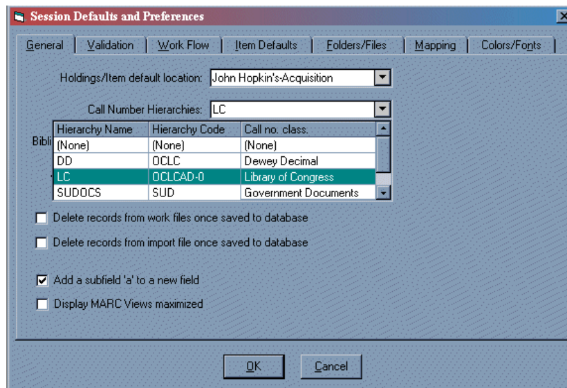
Figure 2-37. Selecting a call number hierarchy
