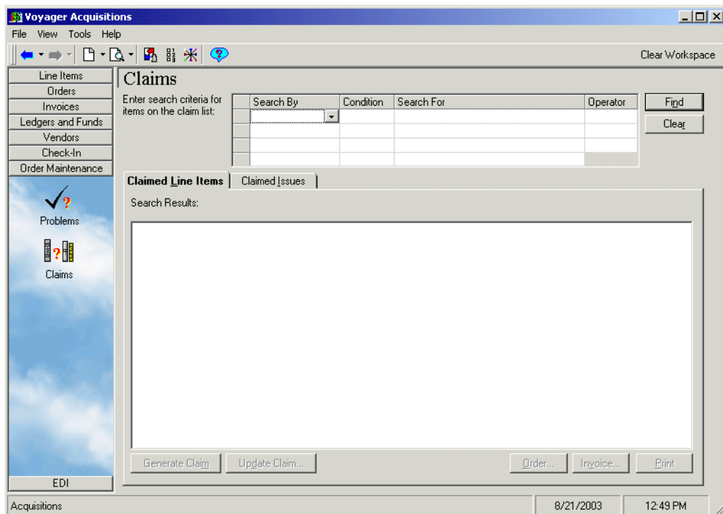
Figure 11-11. Claims workspace
