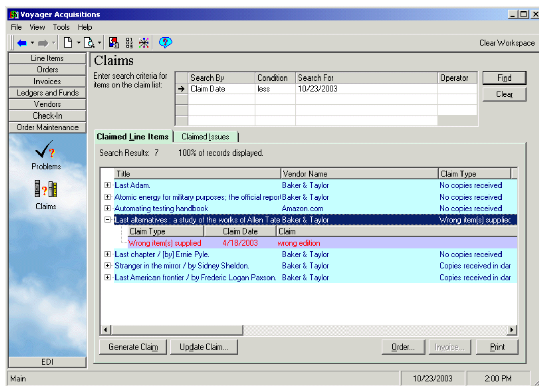
Figure 11-2. Claims workspace
