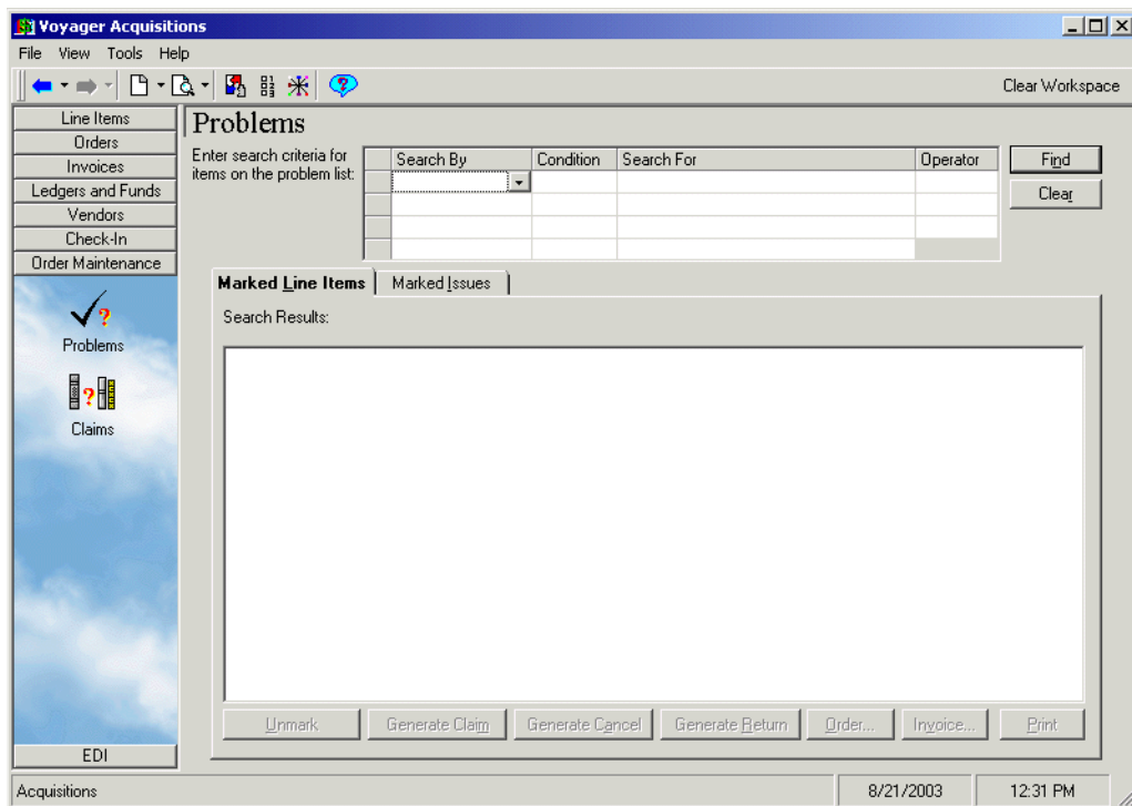
Figure 11-8. Problems workspace
